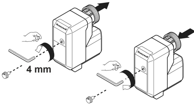
Fig. 6. Manual operation
