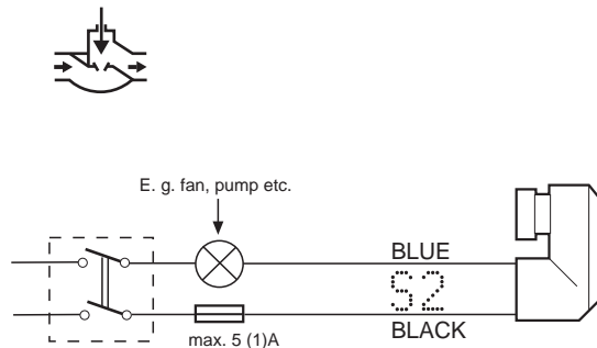
Fig. 11. Electric wiring of auxiliary switch
