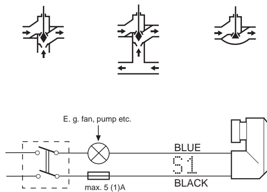
Fig. 12. Electric wiring of auxiliary switch
