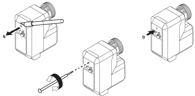
Fig. 9. Adjustment of auxiliary switch S2
