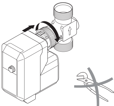
Fig. 3. Mounting the actuator
