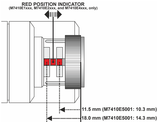
Fig. 7. Movement of the actuator stem (view from above)
