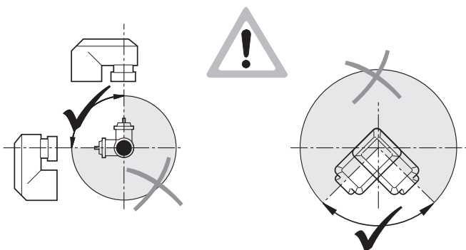
Fig. 1. Mounting positions
