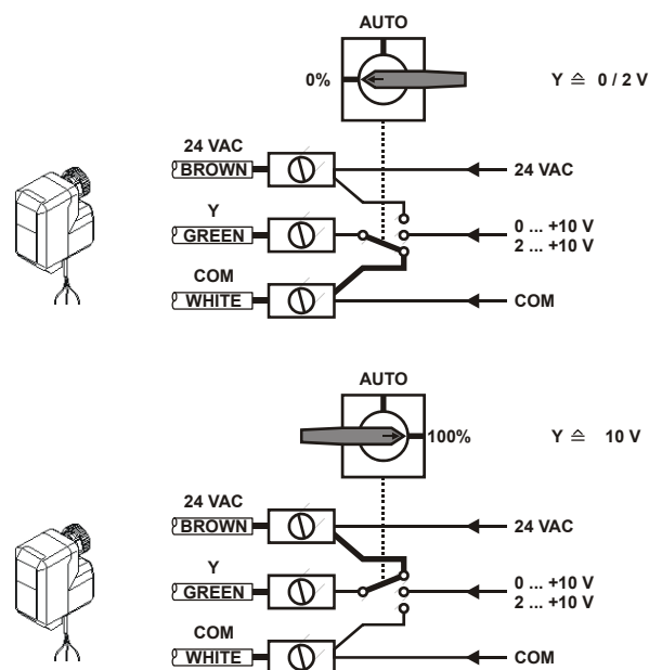
Fig. 5. Connection of input switch
