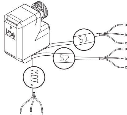
Fig. 8. Auxiliary switch cables
